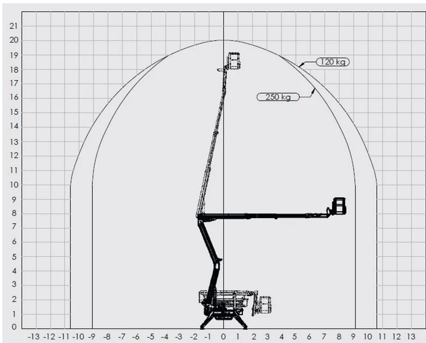
WERKDIAGRAM 20 METER RUTHMANN BLUELIFT SA 20
